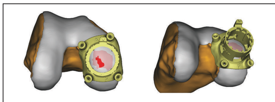
Figure 2. Examples from a “Final Design”. The shape and position of the MRI-based individualized 3D-printed guide instrument are shown.
